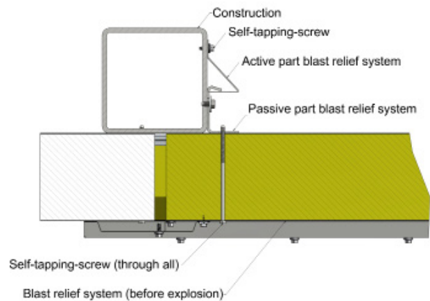
Detail D.1
