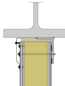
Top section
